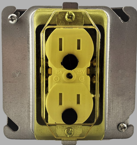
DCP-1P 1 Gang Receptacle Cover w/Pins
